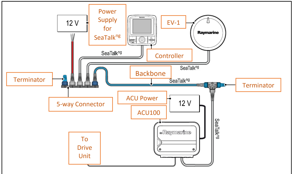
Figure 1 - Typical EV-1 Installation
