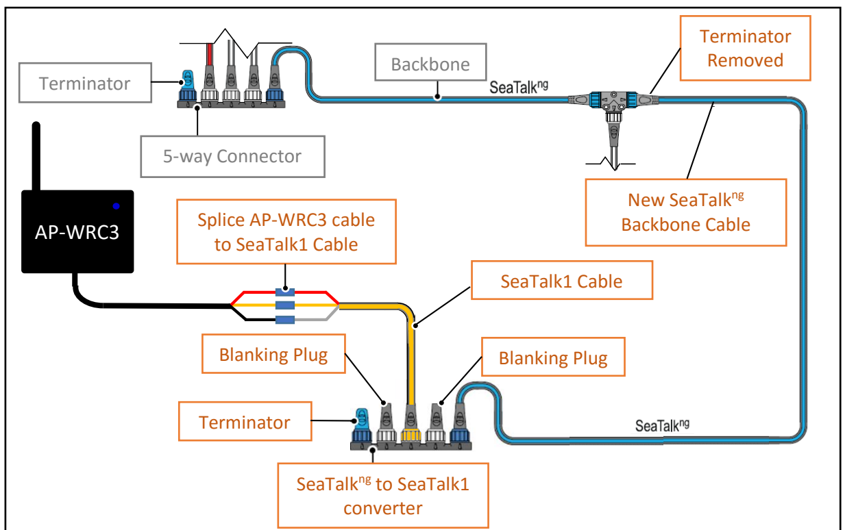
Figure 2 - AP-WRC3 (or AP-WRC3iF) Installation
